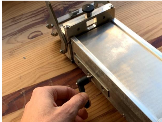
Figure 4: Loosen the telescopic arm clamp lever
