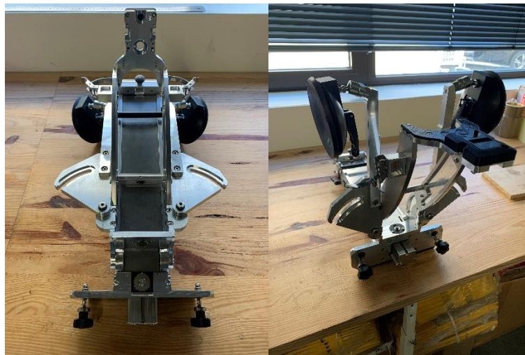
Figure 1: Unfold the chassis
